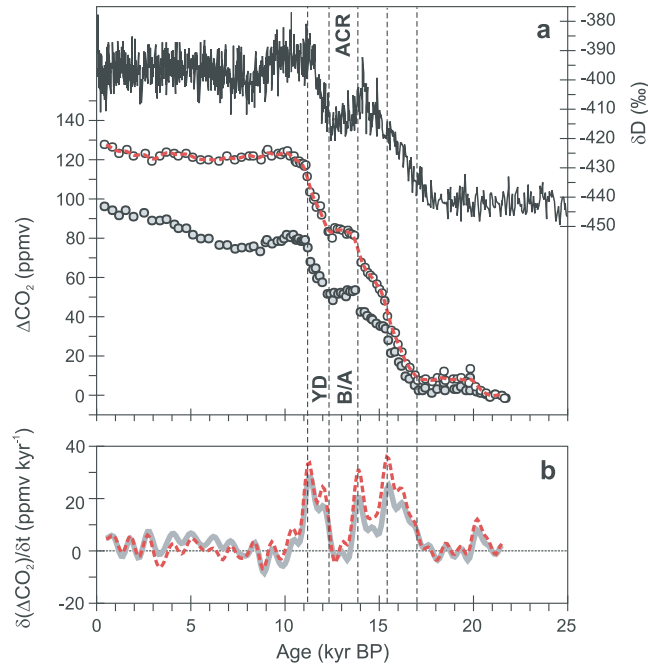
Figure 5. Residual CO 2 “target” record to be accounted for by upper ocean processes. (a) Shown are the dome C δD record [Jouzel et al. , 2001] (solid curve, top) highlighting the relative timing of the Antarctic Cold Reversal (ACR), Bølling/Allerød (B/A), and Younger Dryas (YD) intervals (assigned after Monnin et al. [2001]), observed atmospheric CO 2 changes [Flückiger et al. , 2002; Monnin et al. , 2001] as grey filled circles, and our “residual” CO 2 record as empty circles, formed by subtracting the effects of regrowth of the terrestrial biosphere and reef buildup (assuming the lower 0.5 \times 10^{17} mol C carbonate deposition scenario), along with the effect of dilution of dissolved species in the ocean resulting from the melting of the ice sheets and sea level rise [Fairbanks, 1989]. Both data sets are now plotted as a change relative to LGM values. It should be noted that to form the CO 2 residual, the influences on CO 2 of changes in the terrestrial biosphere, neritic carbonate deposition, and sea level are not subtracted individually from the observed record (which would assume a linear, additive response), but by subtracting the results of a model integration with all three forcings acting simultaneously. Shown as a red dotted line in the residual CO 2 record interpolated at 0.1 kyr intervals and FFT smoothed, which forms the basis of the rate-of-change curve in Figure 5b. (b) Rate of change of observed (thick gray line) and “residual” (dashed red line) CO 2 since the LGM. The timing of the sharp spikes at 13.8 and 11.1 kyr BP, corresponding to discernable “jumps” in observed CO 2 record (Figure 5a) appear to be coincident with prominent warming transitions in the North Atlantic (not shown). It is therefore likely that they reflect the effect of Northern Hemisphere ocean surface temperature increases, sea ice retreat, and/or a rapid strengthening of the Atlantic overturning circulation.
